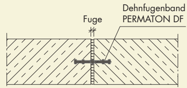
Dehnfuge in Bodenplatte
